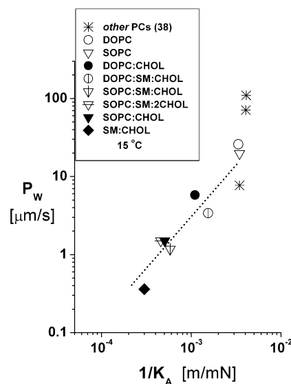
FIGURE 6 Values of water permeability P_w measured at 15°C are plotted as functions of the area compressibility 1/K_A as defined by the elastic-stretch moduli at 15°C in Fig. 2 (Table 1). Also included are data for other fluid-PC bilayers (taken from Rawicz et al. (35) and Olbrich et al. (38)). The dashed-dotted line was added to highlight the correlation between permeability and area compressibility among the phospholipid/CHOL systems.
